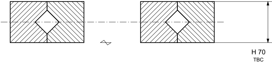
LOCAL SECTION A-A / AXIS GAP SHORTENED Local scale 0.25:1; rolling elements and interfaces schematic.
