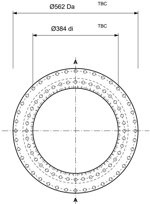
LOCAL SECTION A-A / AXIS GAP SHORTENED Local scale 0.25:1; rolling elements and interfaces schematic.
