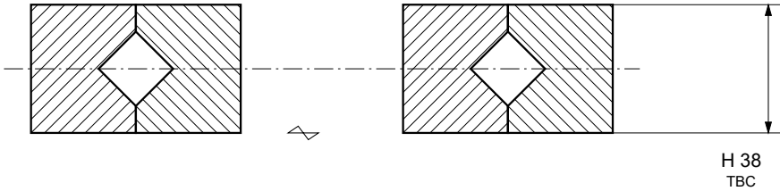
LOCAL SECTION A-A / AXIS GAP SHORTENED Local scale 0.5:1; rolling elements and interfaces schematic.
