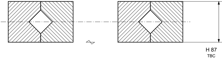
LOCAL SECTION A-A / AXIS GAP SHORTENED Local scale 0.25:1; rolling elements and interfaces schematic.
