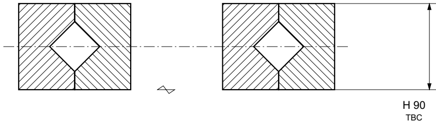
LOCAL SECTION A-A / AXIS GAP SHORTENED Local scale 0.25:1; rolling elements and interfaces schematic.
