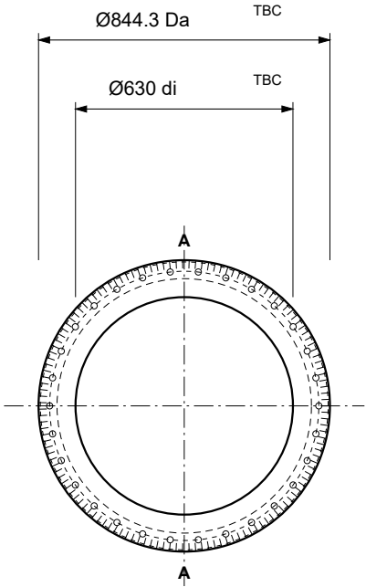
LOCAL SECTION A-A / AXIS GAP SHORTENED Local scale 0.25:1; rolling elements and interfaces schematic.
