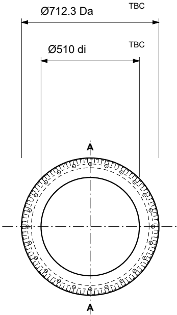
LOCAL SECTION A-A / AXIS GAP SHORTENED Local scale 0.25:1; rolling elements and interfaces schematic.
