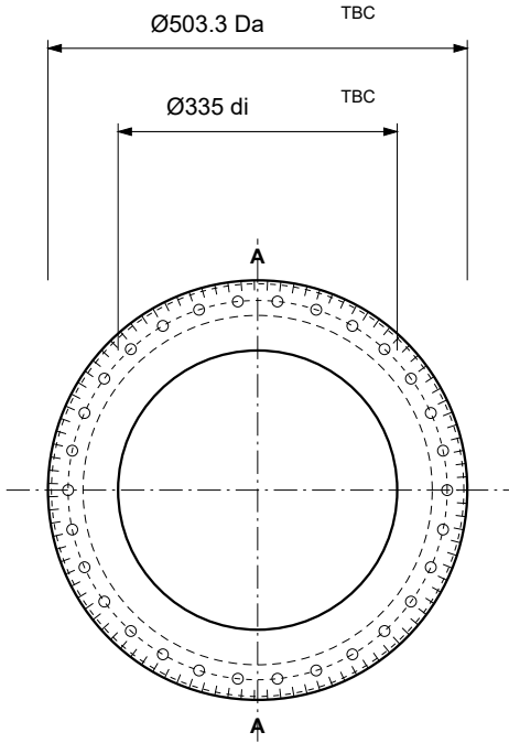
LOCAL SECTION A-A / AXIS GAP SHORTENED Local scale 0.25:1; rolling elements and interfaces schematic.
