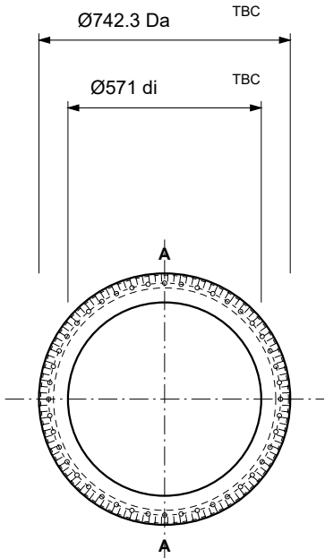
LOCAL SECTION A-A / AXIS GAP SHORTENED Local scale 0.25:1; rolling elements and interfaces schematic.
