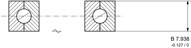
LOCAL SECTION A-A / AXIS GAP SHORTENED Local scale 2:1; rolling elements and interfaces schematic.
